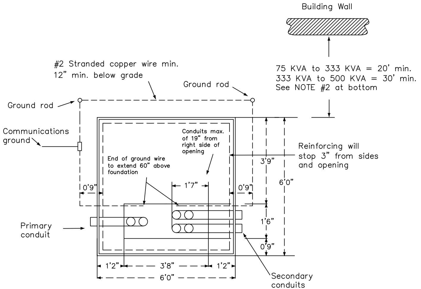
PLAN
